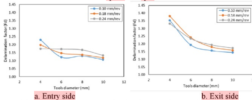
Figure 17 Correlation between delamination factor and tool's diameter on the spindle speed 1420 rpm
