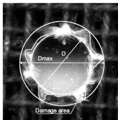
Figure 5. Delamination measurement method, [24].
