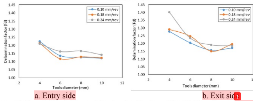
Figure 16 Correlation between delamination factor and tool's diameter on the spindle speed 443 rpm
