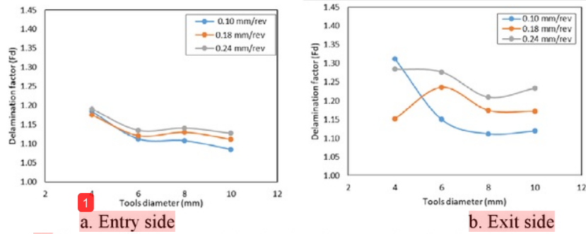
Figure 15 Correlation between delamination factor and tool's diameter on the spindle speed 93 rpm
