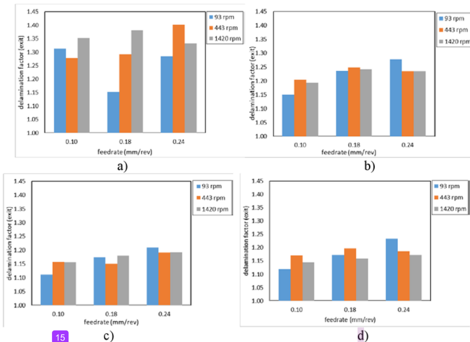
Figure 14 Effect of spindle speed concerning feed rate on delamination factor at the exit side, with the tool's diameter: a) 4 mm; b) 6 mm; c) 8 mm and d) 10 mm
