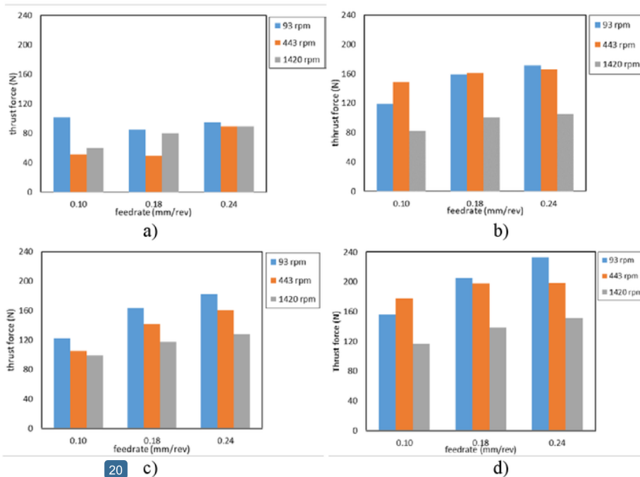
Figure 10 Correlation between thrust force and feed rate at the tool's diameter: a) 4 mm; b) 6 mm; c) 8 mm; d) 10 mm
