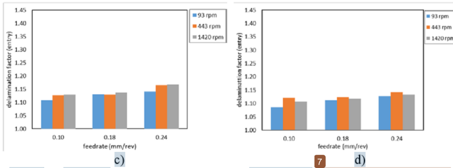
Figure 13 Effect of spindle speed concerning feed rate on delamination factor at the entry side, with the tool's diameter: a) 4 mm; b) 6 mm; c) 8 mm and d) 10 mm
