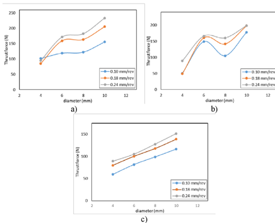
Figure 11 Correlation between thrust force and tools diameter on the spindle speed: a) 93 rpm; b) 443 rpm; c) 1420 rpm.
