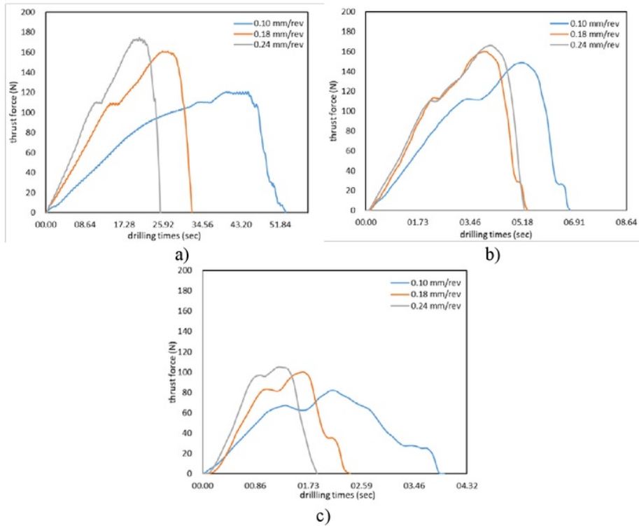
Figure 7 Thrust force over drilling cycle of tools diameter 6 mm at the spindle speed: a) 93 rpm; b) 443 rpm; c) 1420 rpm
