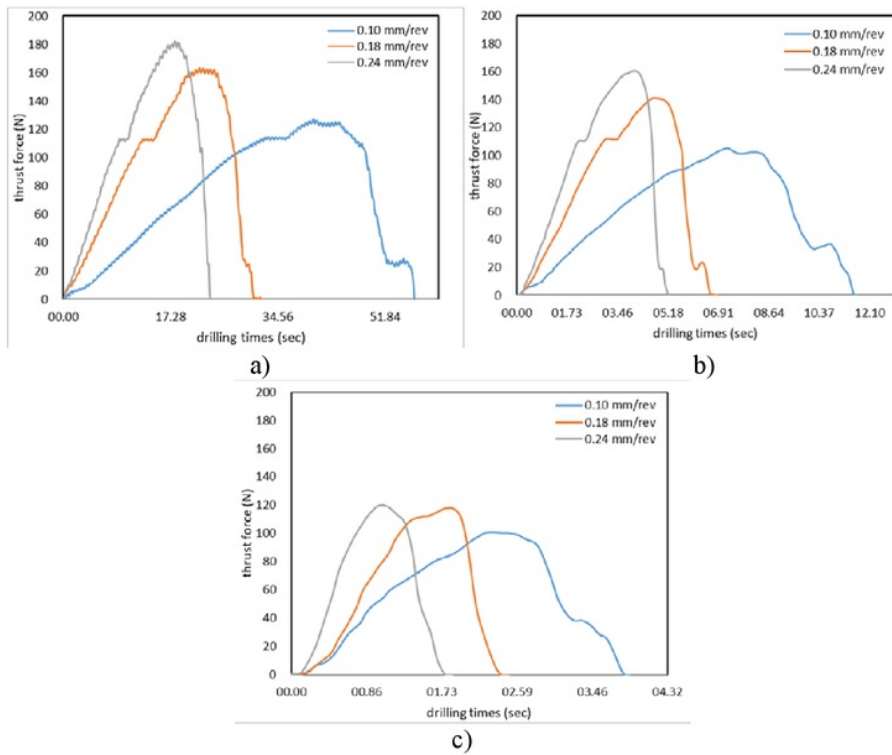
Figure 8 Thrust force over drilling cycle of tools diameter 8 mm at the spindle speed; a) 93 rpm; b) 443 rpm; c) 1420 rpm
