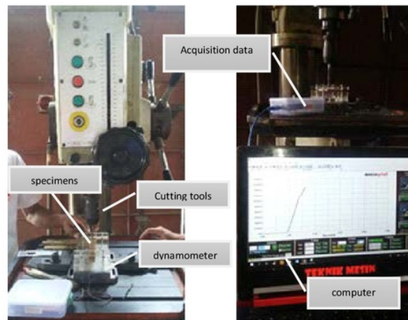
Figure 4. Experimental set-up
