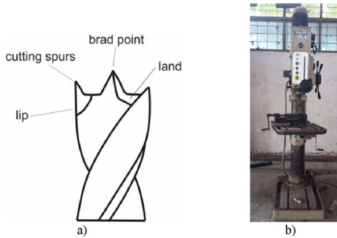
Figure 3. a) “Brad & spur” drill’s detail; b) Pillar drill TCA-35 ERLO
